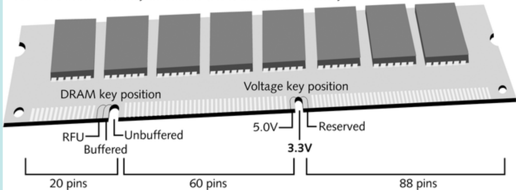
Figure 6-6 The positions of two notches on a DIMM identify the type of DIMM and the voltage requirement, and also prevent the wrong type from being installed on the motherboard
